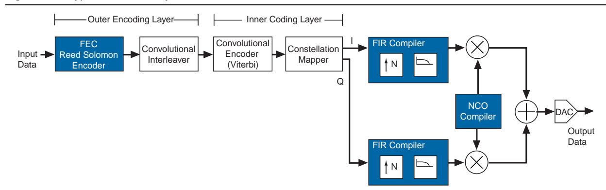
Figure 1-3. Typical Modulator System
