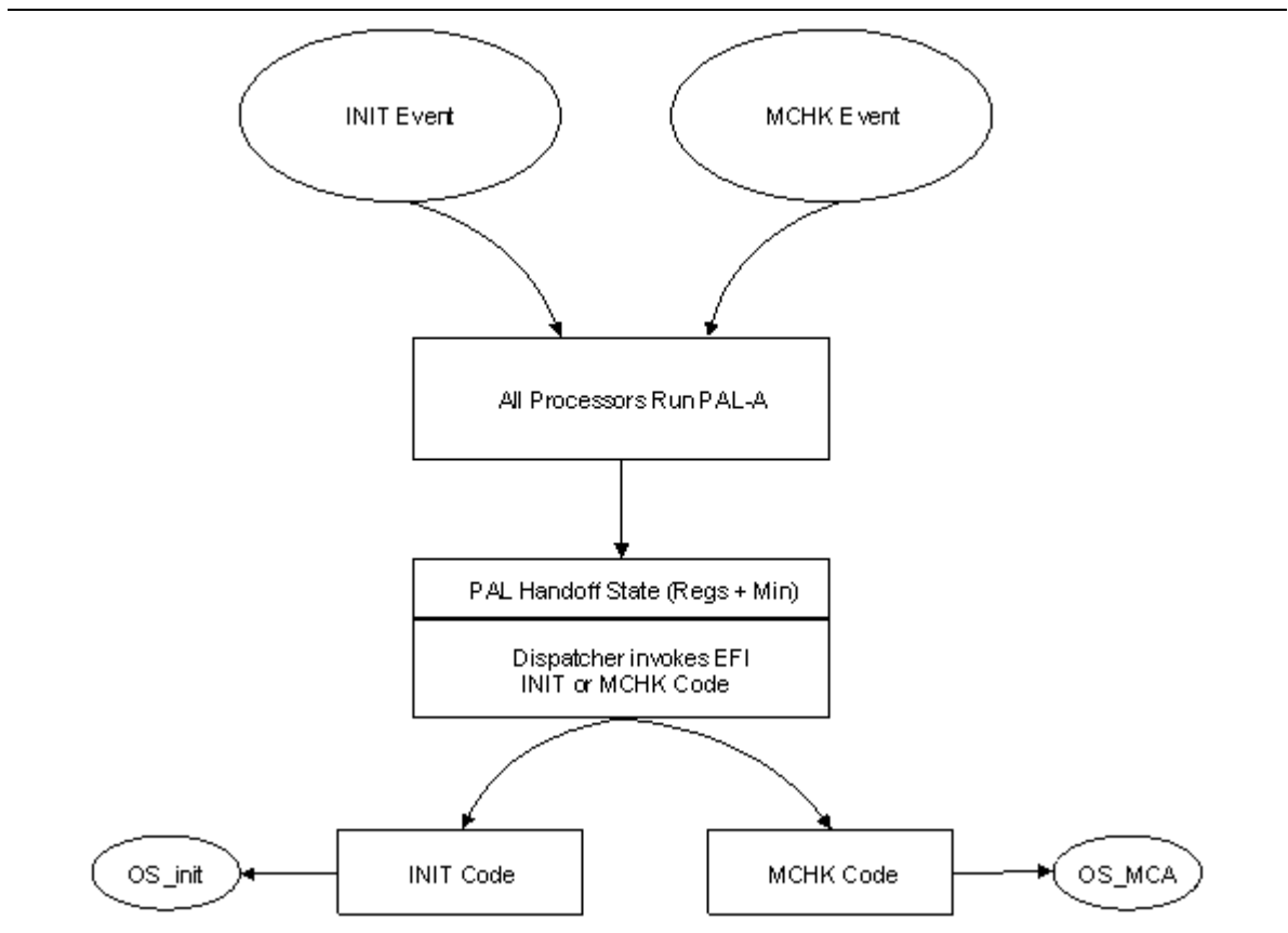
Figure 13-1. Itanium Processor Boot Path (INIT and MCHK)
