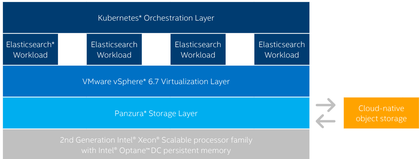
Figure 1. The phoenixNAP Elasticsearch* Service enables object storage to be used for scale-out storage of metadata which can be searched and analyzed using Elasticsearch. The solution is based on the 2nd generation Intel® Xeon® Scalable processor family with Intel® Optane™ DC persistent memory.
