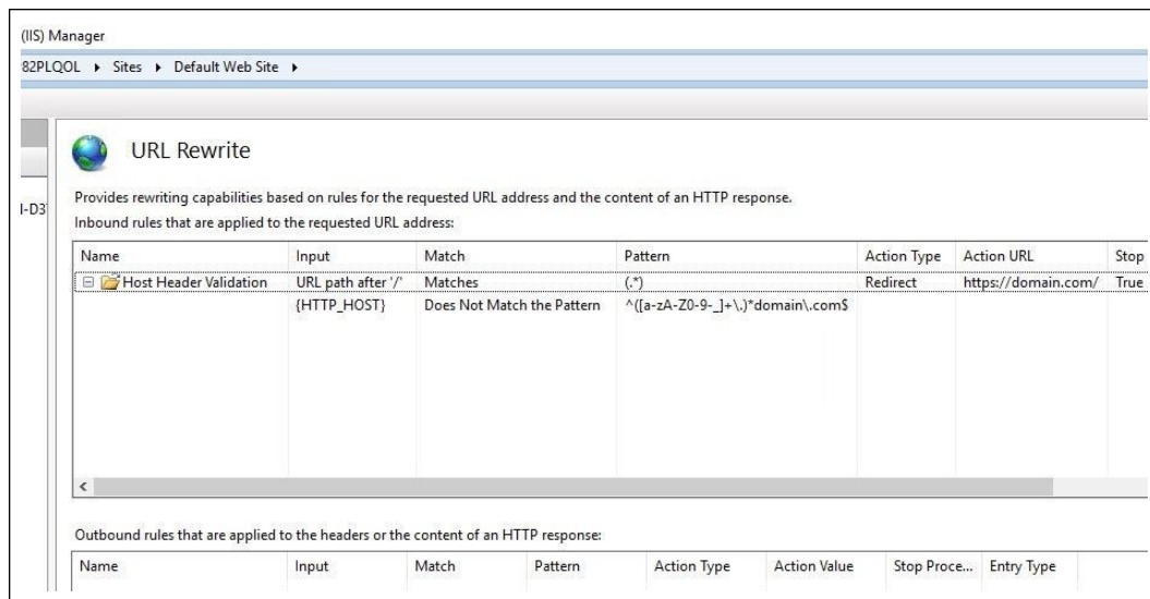
Figure 1. URL Rewrite
