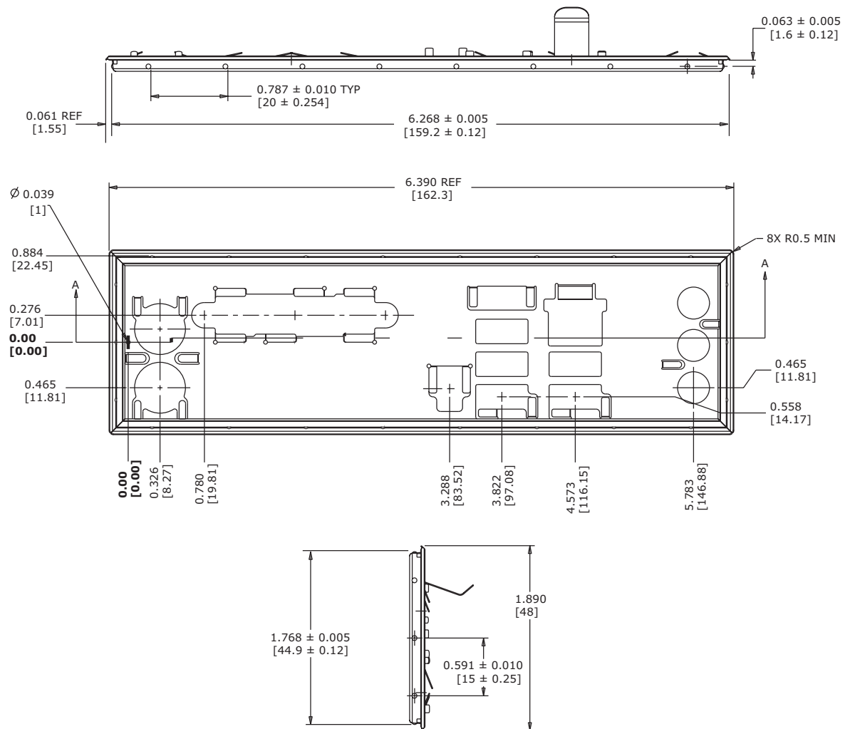
Figure 22. I/O Shield Dimensions
