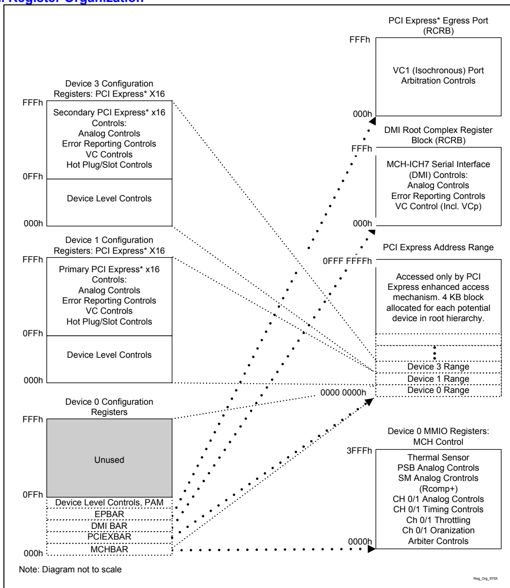
Figure 3-2. Register Organization
